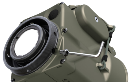
Screw in the clamping screw
